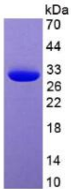
Figure 2. SDS-PAGE
